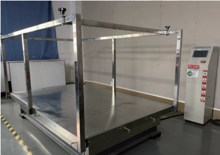
VIBRATION TEST
